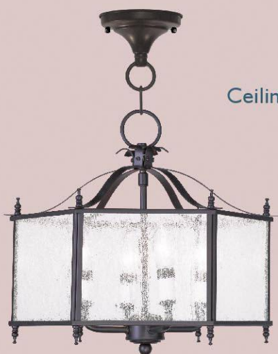
4399-07 Chain Hang 15.5" Dia x 13" H With Seeded Glass
